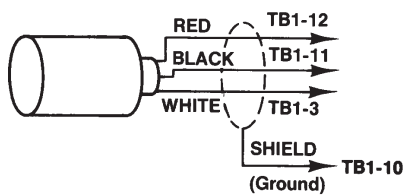
HFBG (High Frequency Pulse Generator)
